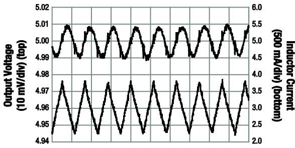
Time (2 μs/div)
