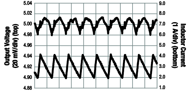
Time (2 μs/div)
