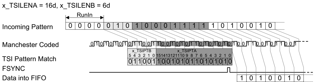
Figure 27 16-Bit TSI Mode
