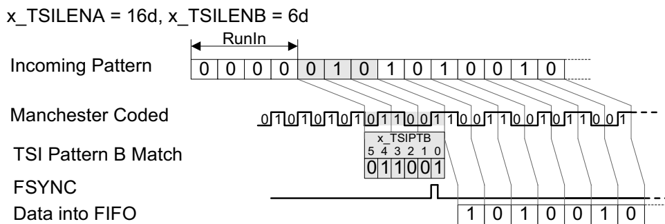
Figure 28 8-Bit Parallel TSI Mode
