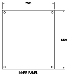
INNER PANEL
