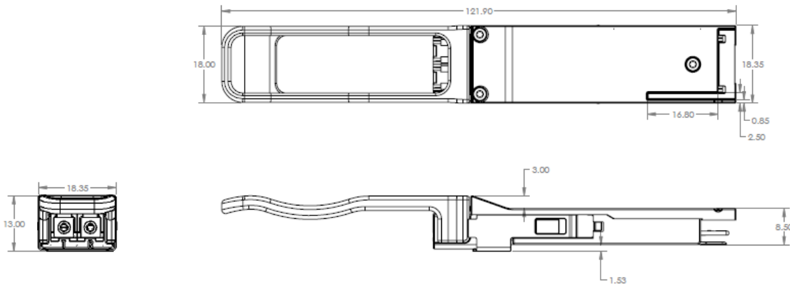
Figure 2 – FTL4E1Q mechanical drawing
