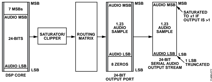
Figure 69. 24-Bit Serial Output Example
