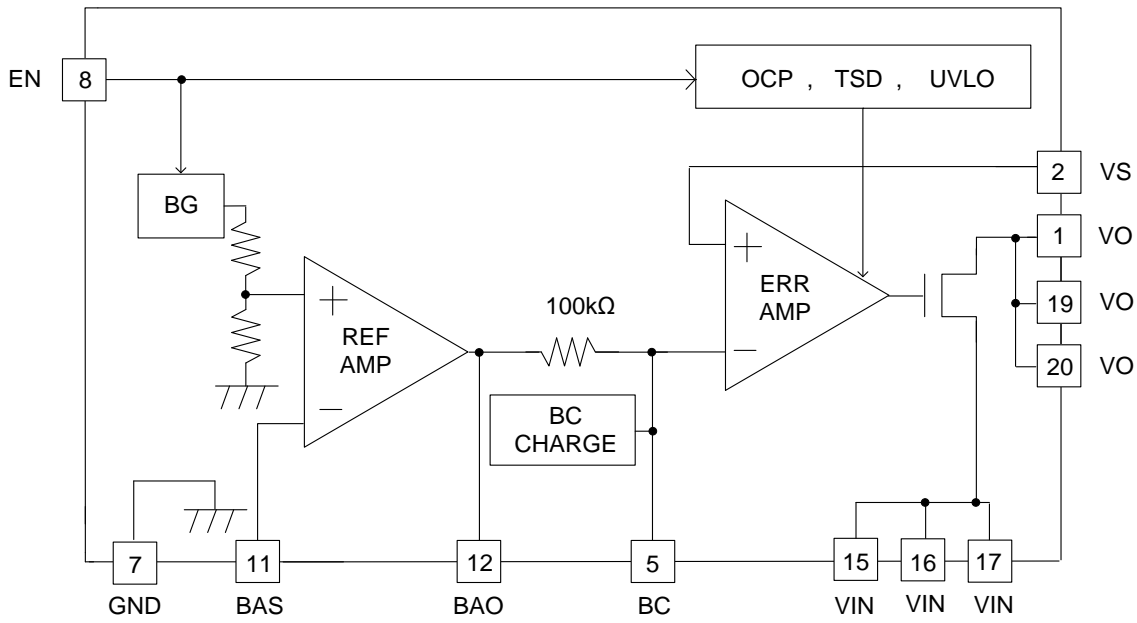
Figure 3. Block Diagram
