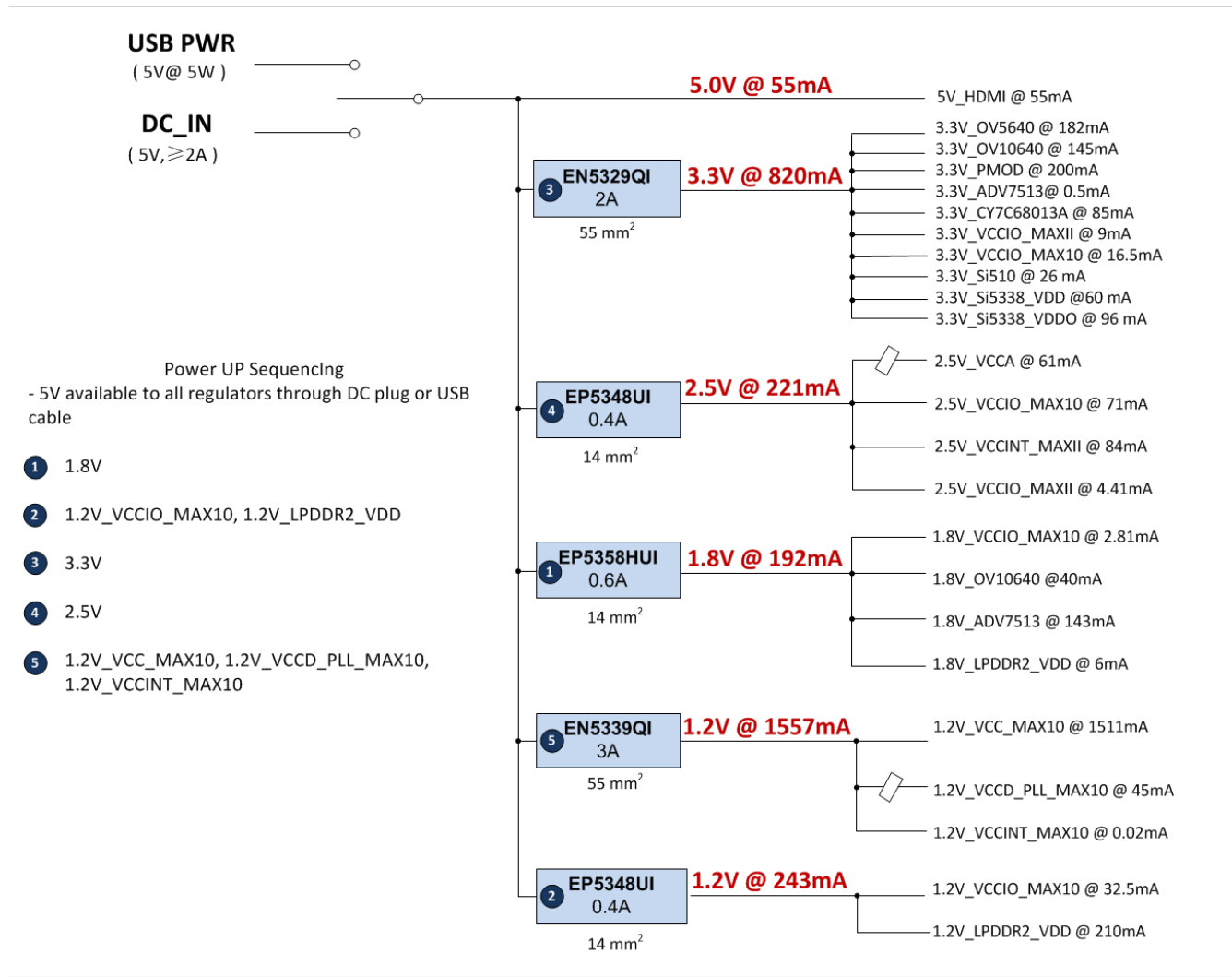
Figure 3-5: Power Tree
