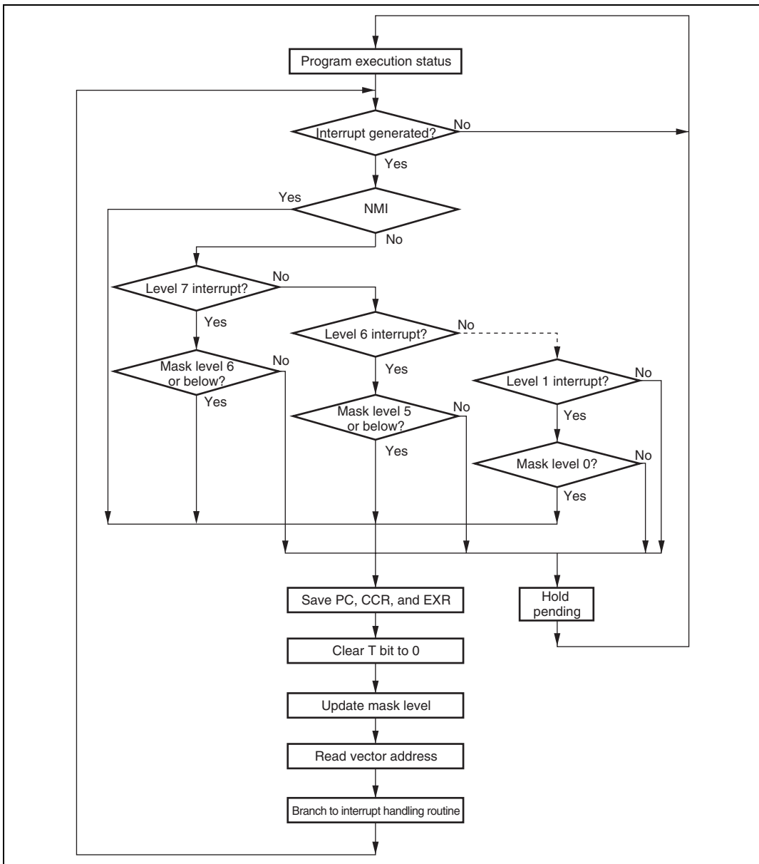
Figure 5.4 Flowchart of Procedure Up to Interrupt Acceptance in Control Mode 2
