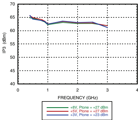
Input Third Order Intercept
