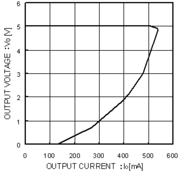
Fig.5 Load Regulation
