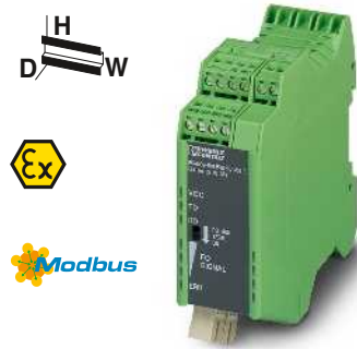
RS-485 2-wire fiberglass (multi mode and single mode)
