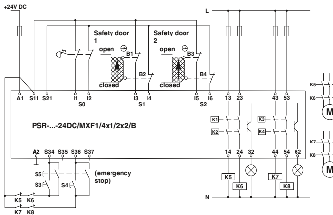
Emergency stop and safety door monitoring
