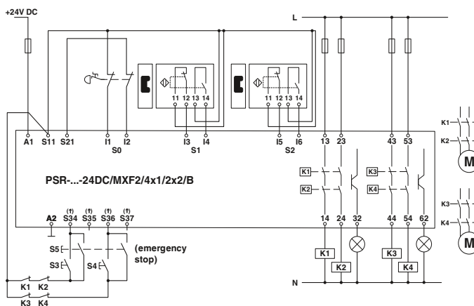
Emergency stop and magnetic switch monitoring
