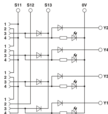
Block diagram
