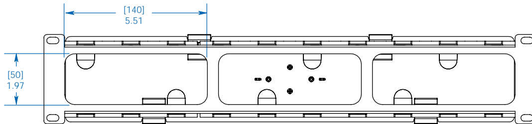
REAR VIEW
