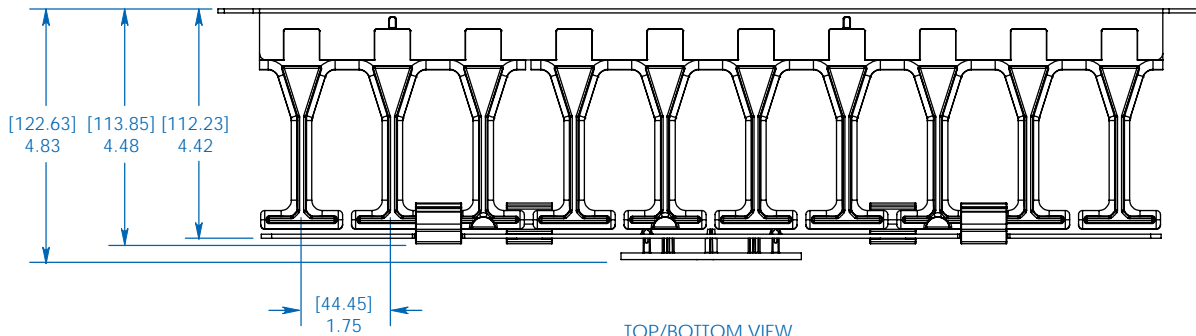
TOP/BOTTOM VIEW
