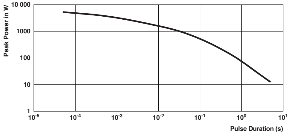
Pulse performance after a rectangular pulse of defined duration is applied
