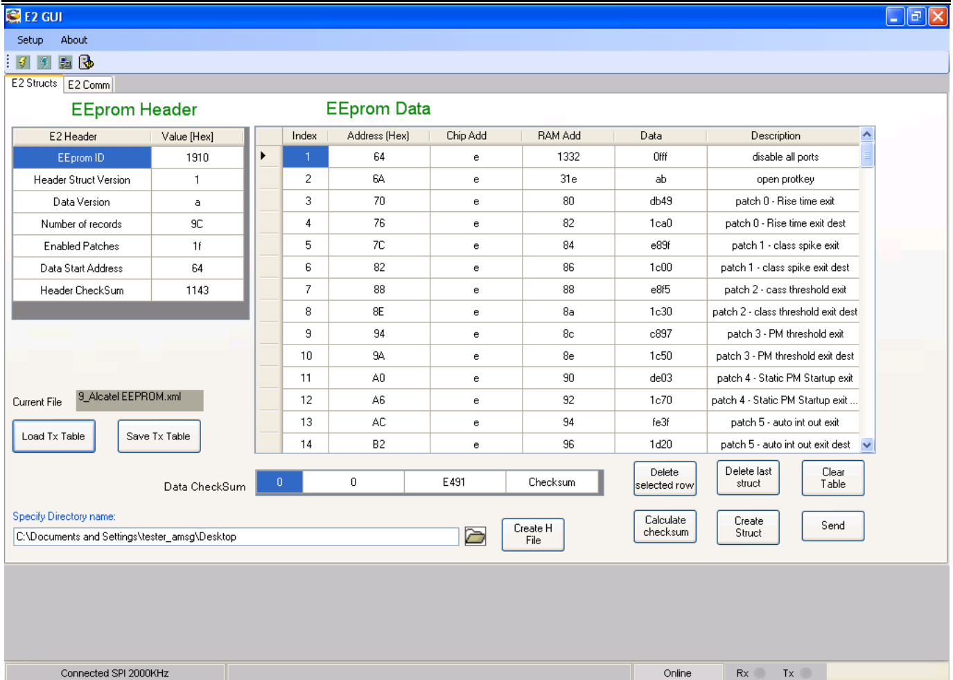
Figure 18: E2 GUI
